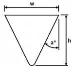
Wedge Wire Cross Section
