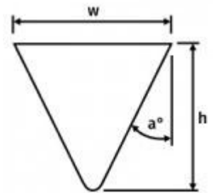
Wedge Wire Cross Section
