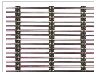
Gladstone PC 42/3 architectural mesh installed as balustrading on White Horse Bridge, Wembley.
